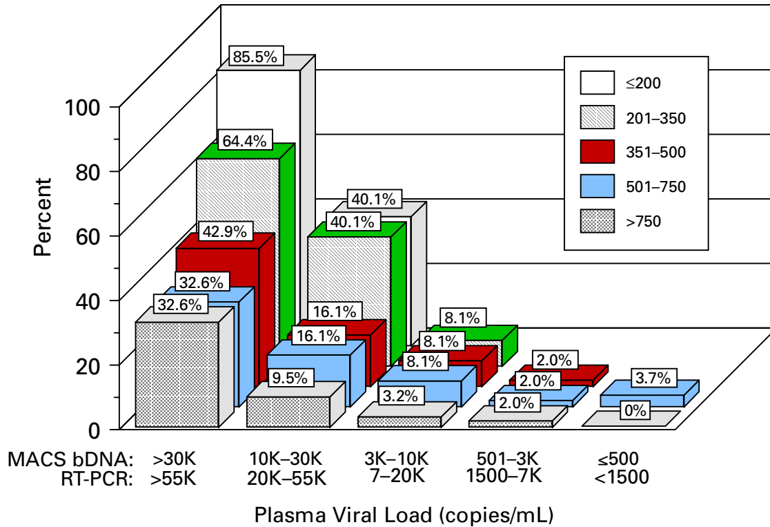
FIGURE 1. Likelihood of developing AIDS within 3 years*
