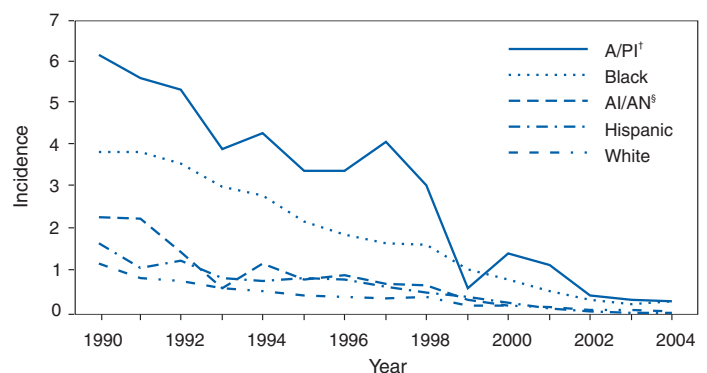
FIGURE 3. Reported acute hepatitis B incidence* among persons aged <19 years, by race/ethnicity and year — United States, 1990–2004
