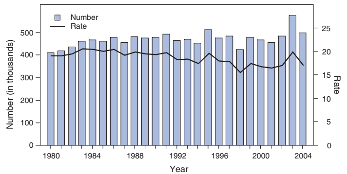
FIGURE 3. Number and rate* of asthma† hospital discharges, by year — United States, 1980–2004
