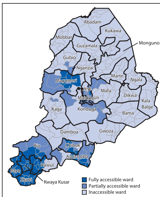
FIGURE 1. Accessibility of local government areas to polio eradication program personnel, by ward — Borno State, Nigeria, September 2015
