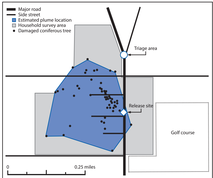
FIGURE. Anhydrous ammonia release site, estimated plume location based on damaged coniferous trees,* and area covered by the household survey for the assessment of chemical exposures — Lake County, Illinois, April 2019
