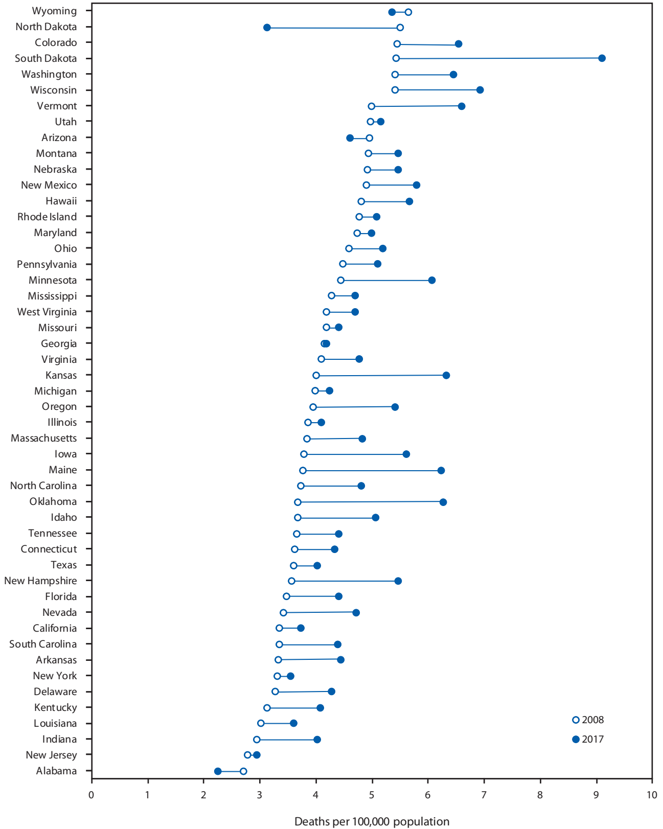
FIGURE. Age-adjusted* rate of traumatic brain injury–related deaths caused by unintentional falls, by state† — United States, 2008 and 2017
