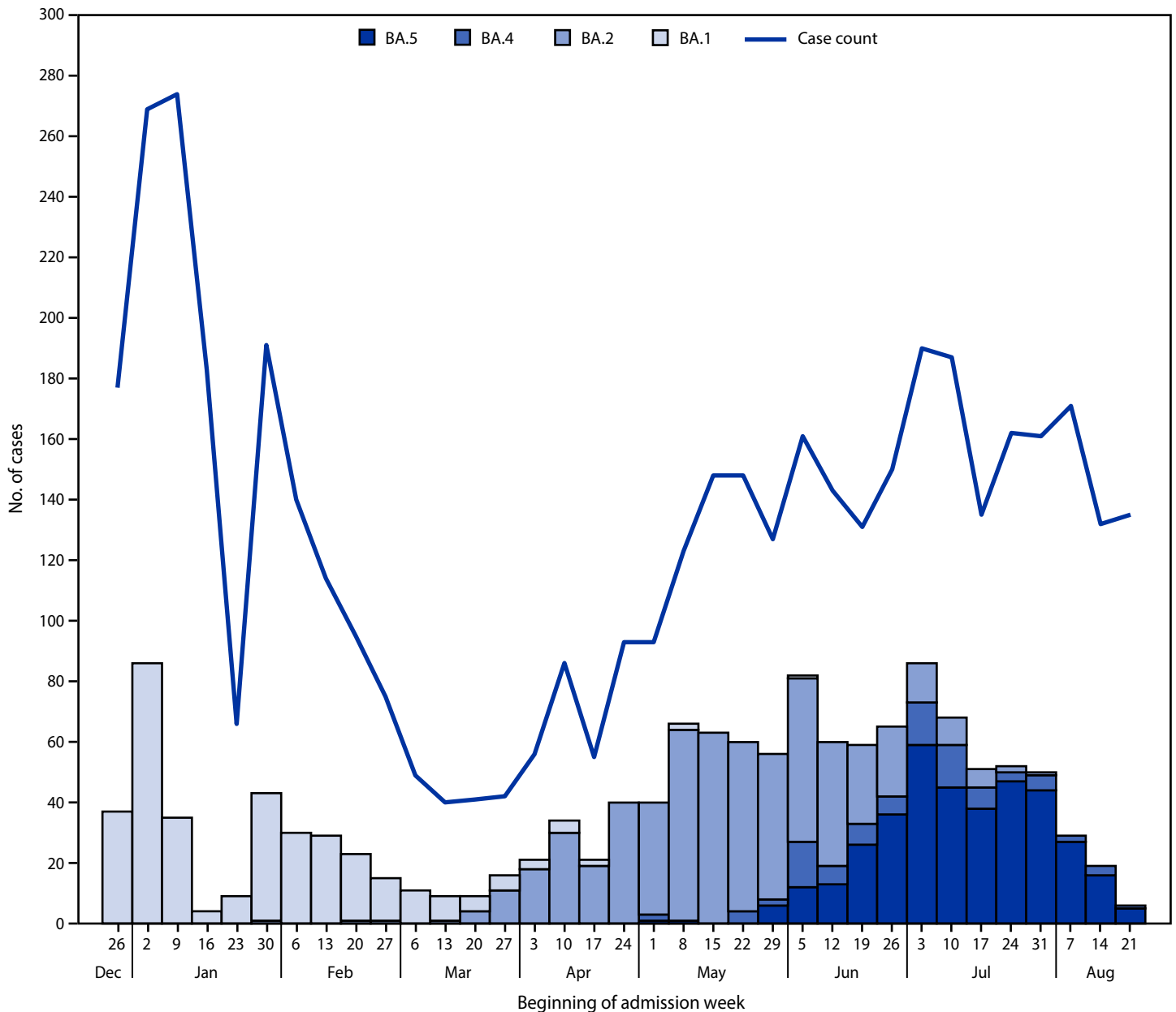
FIGURE. Numbers of COVID-19 cases* and SARS-CoV-2 whole genome–sequenced lineages †,§,¶ among immunocompetent adults hospitalized with COVID-19 — IVY Network, 21 hospitals in 18 U.S. states,** December 26, 2021–August 24, 2022 ††
