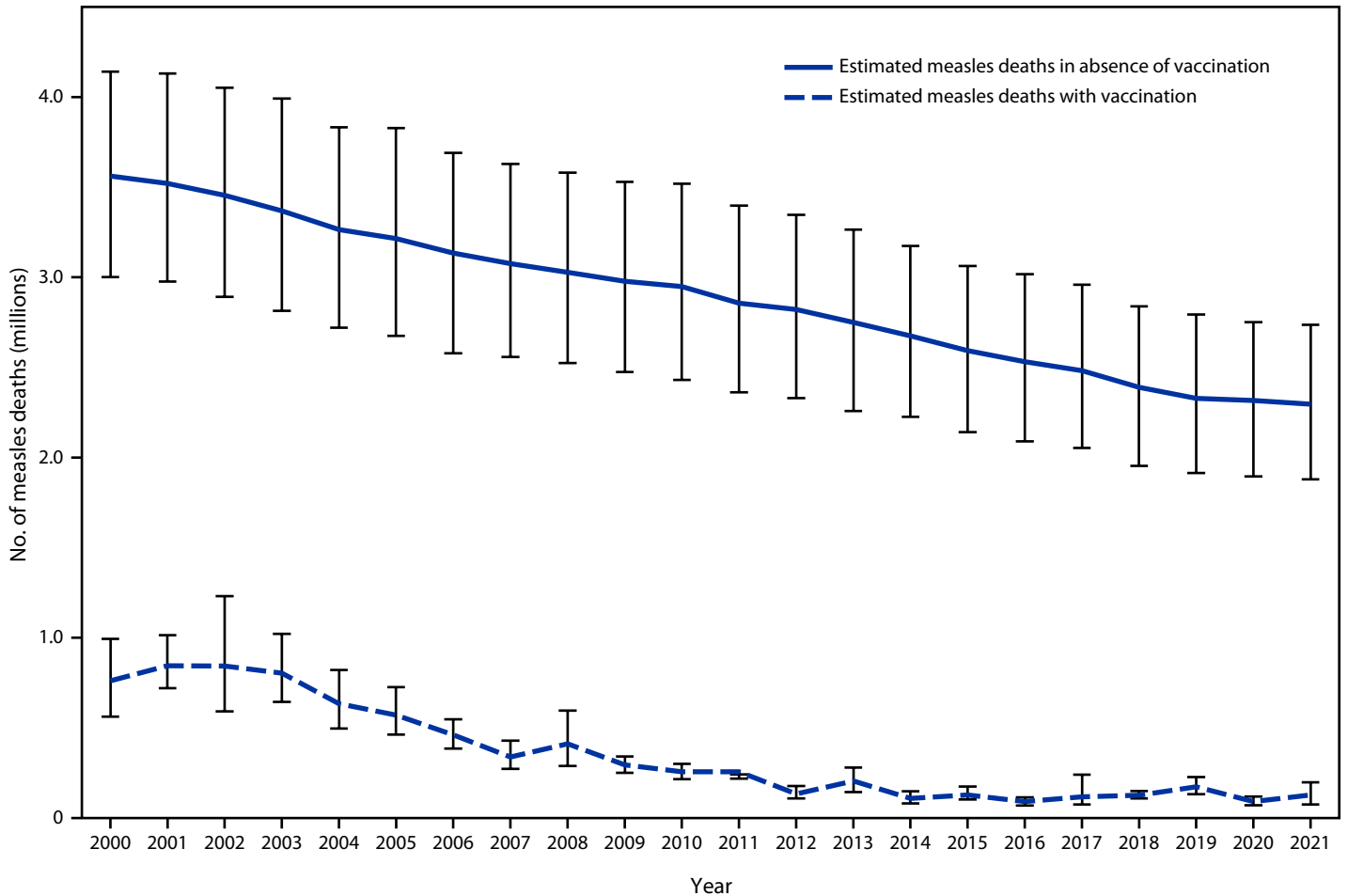
FIGURE. Estimated number of annual measles deaths with measles vaccination and in the absence of measles vaccination — worldwide, 2000–2021*
