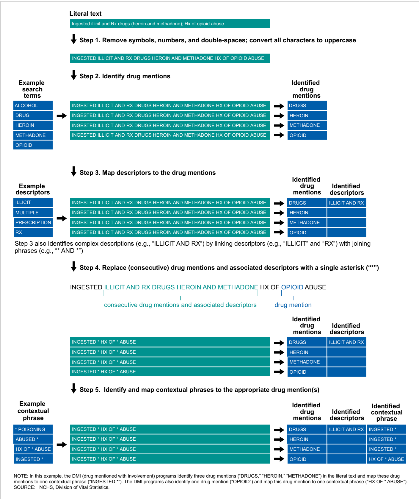
Figure 3. Example of the application of the DMI program logic to the literal text
