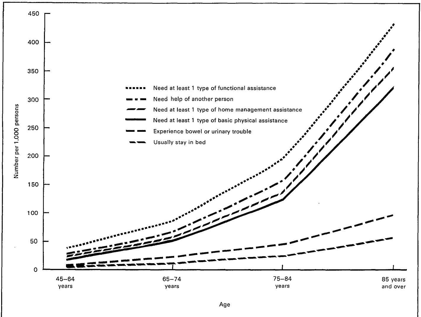
Figure 1. Number of persons who need home care per 1,000 adults 45 years of age and over, by type of measure and age: United States, 1979-80
