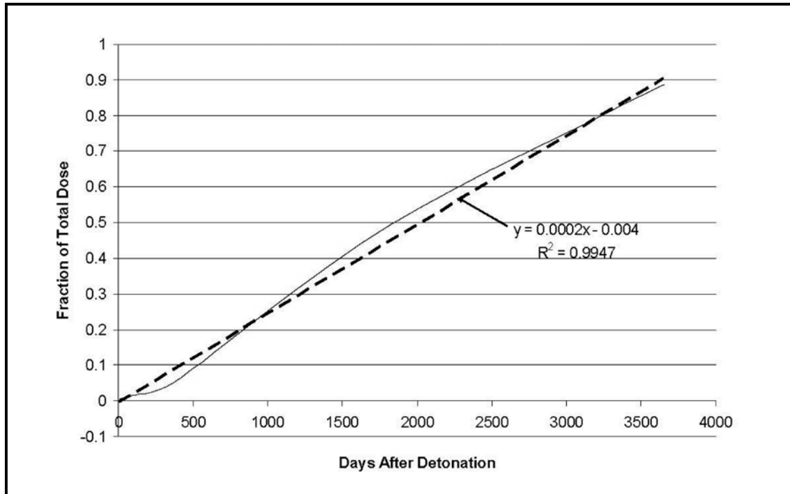
Figure A-3. Little Feller I – ^{90}\text{Sr} fraction of total dose to lungs.
