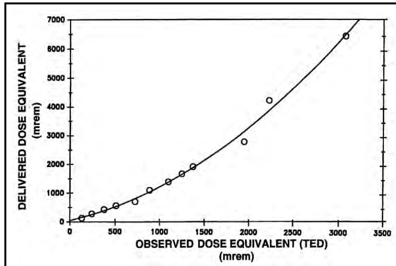
Figure A-6. Electrochemically etched CR-39 dose response (Allen and Schoengold 1995).
