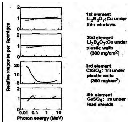
Figure A-2. Panasonic UD-802 energy responses (Allen and Schoengold 1995).
