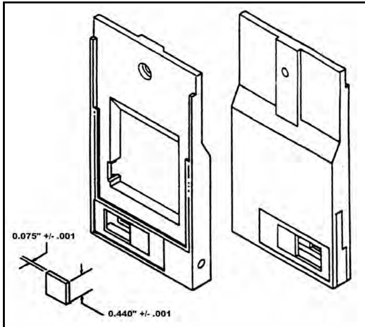
Figure 6-3. REECO badge holder (REECO 1990).
