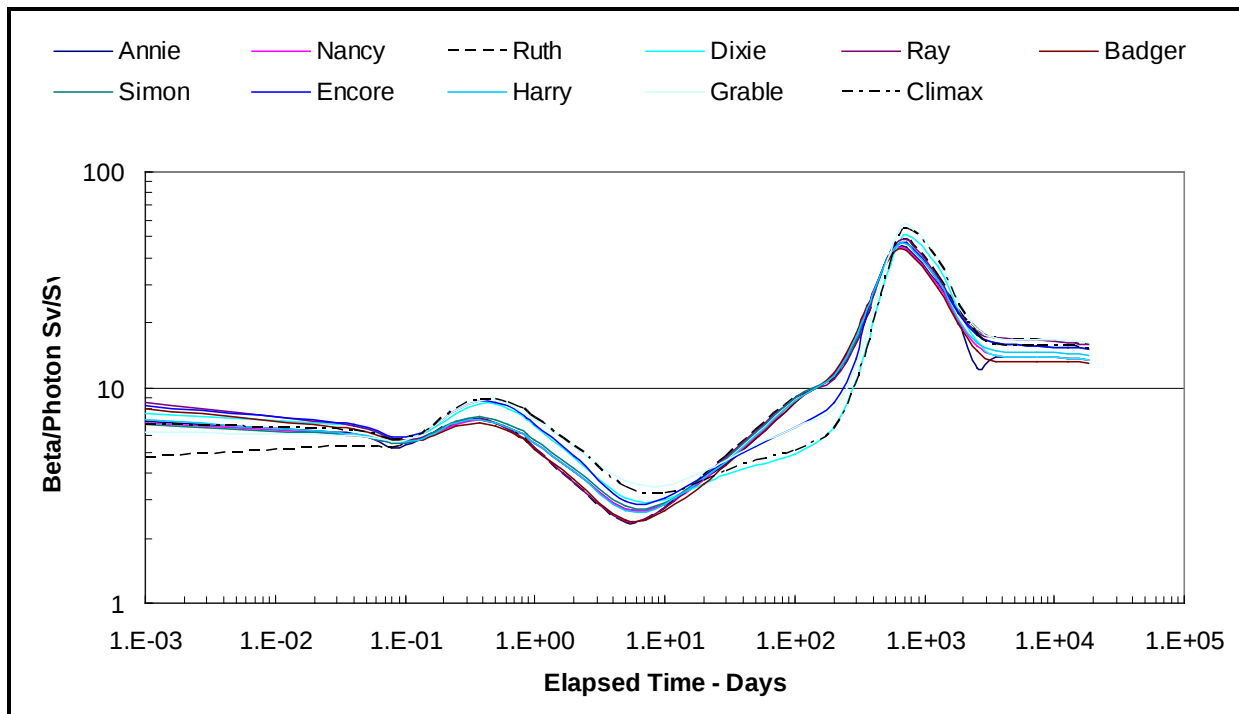
Figure C-2. Calculated beta-photon ratios (Sv/Sv) for skin for 11 atmospheric tests from Operation Upshot-Knothole.
