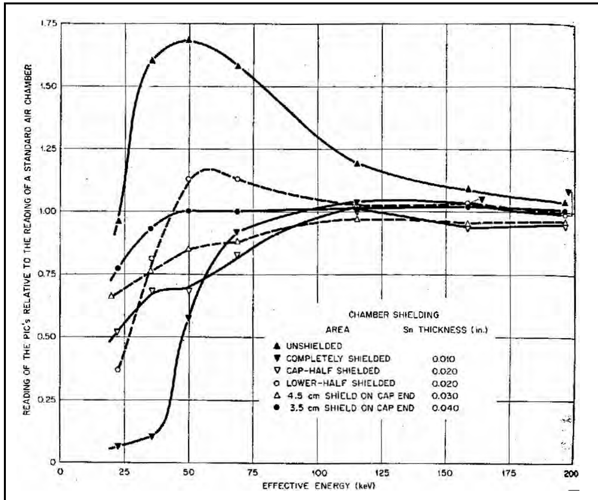
Figure 6-1. X-ray energy dependence of PICs (Sanders, Auxier, and Cheka 1959).
