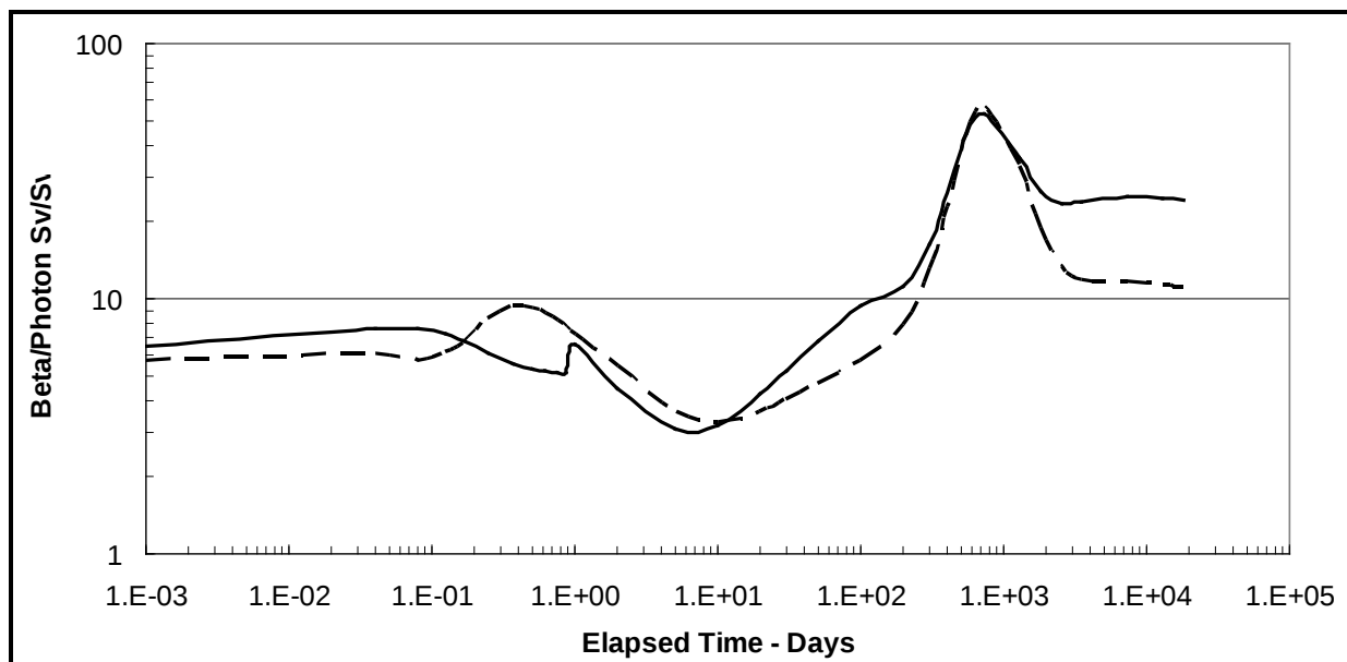
Figure C-3. Calculated beta-photon ratios (Sv/Sv) for skin for nuclear rockets and ramjet test effluents.
