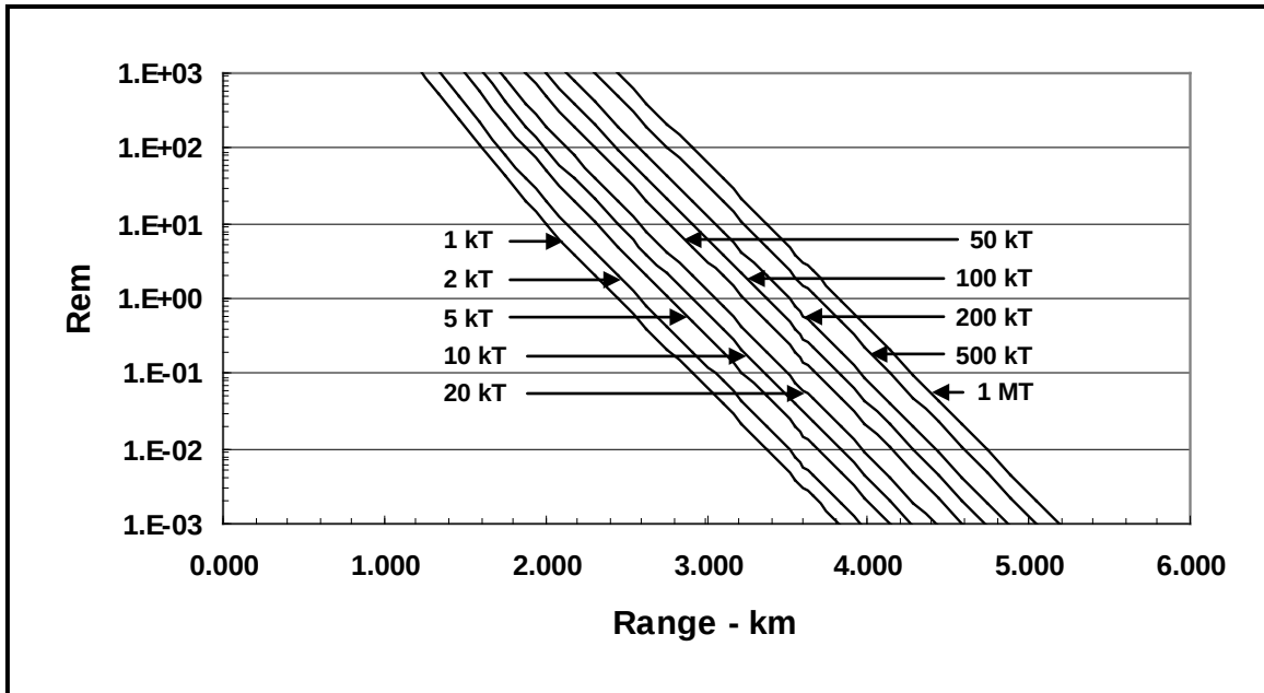
Figure D-4. Neutron dose equivalent as a function of slant range for atmospheric detonations with a range of weapon yields.
