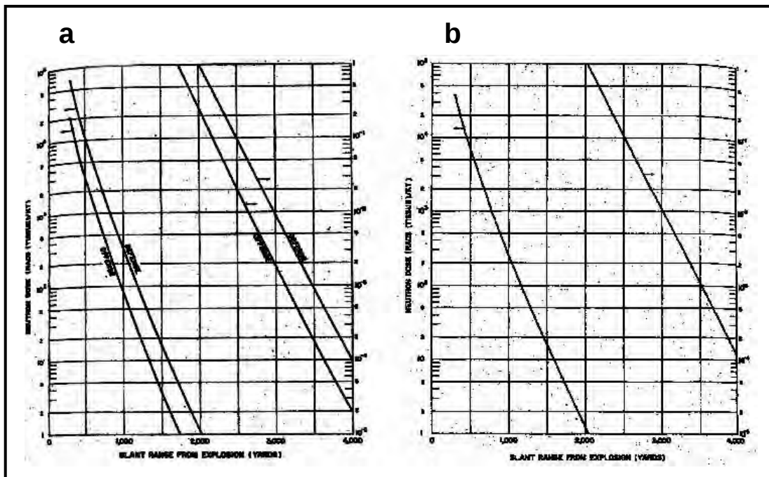
Figure D-2. Initial neutron dose per kT as a function of slant range from (a) fission and (b) thermonuclear air bursts, based on 0.9 normal sea-level air density (Glasstone and Dolan 1977).
