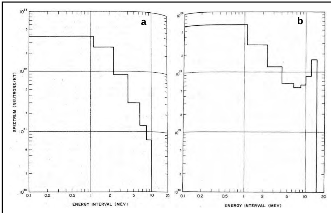
Figure D-1. Neutron spectra for (a) fission weapon and (b) thermonuclear weapon per kiloton total energy yield (Glasstone and Dolan 1977).
