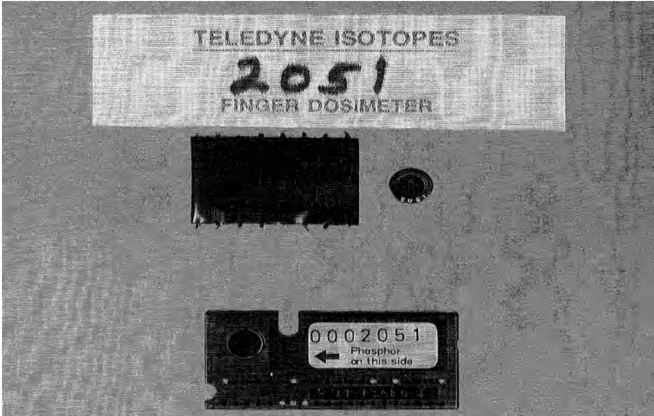
Figure 6-5. Panasonic UD-807 extremity dosimeter (Allen and Schoengold 1995).
