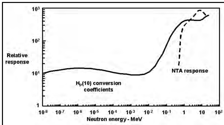
Figure A-3. NTA film neutron energy response (IAEA 1990).
