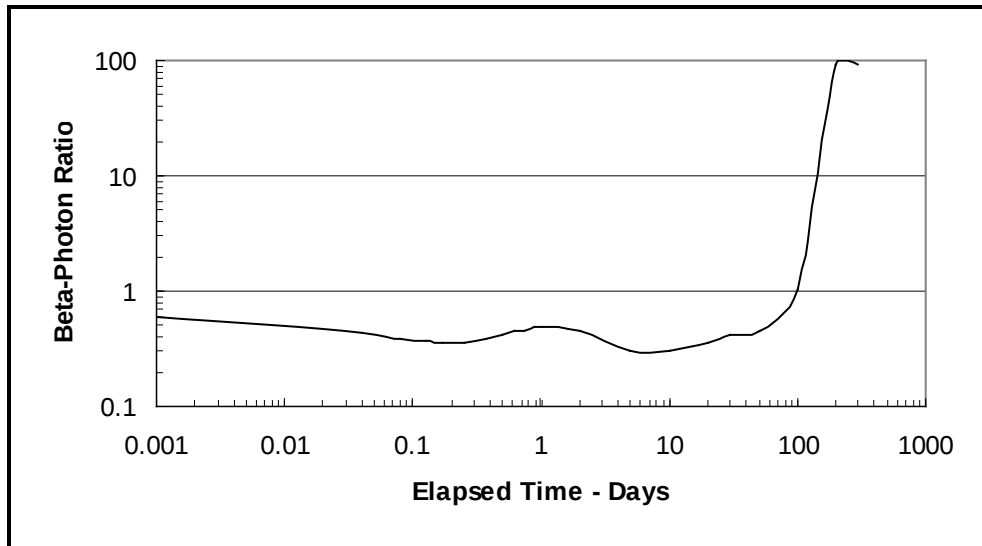
Figure C-4. Calculated beta-photon ratios for immersion in a contaminated semi-infinite cloud—maximum of values from 11 atmospheric test radionuclide inventories.
