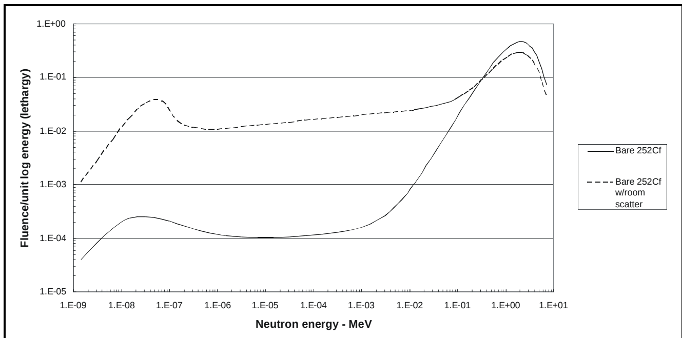
Figure A-7. Lethargy neutron spectra for ^{252}\text{Cf} calibration source with and without room scatter (IAEA 2001).
