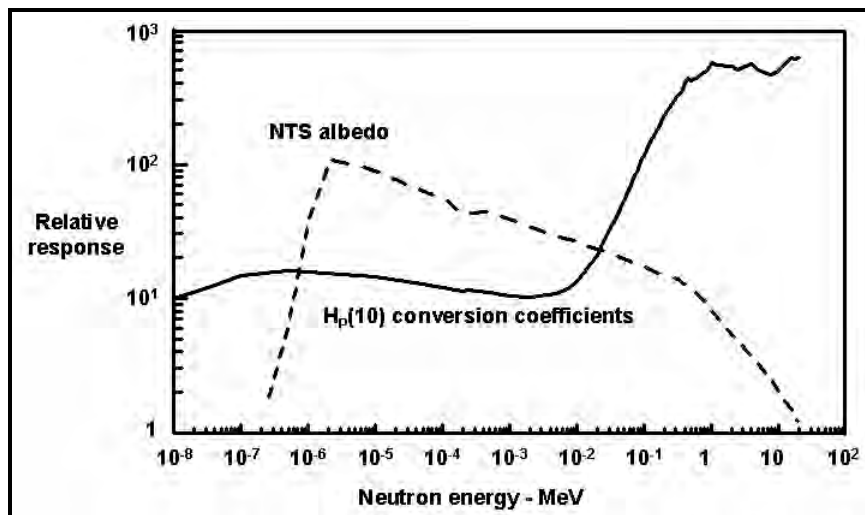
Figure A-4. Neutron energy response of NTS albedo dosimeters (IAEA 1990).
