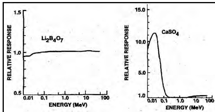
Figure A-1. Typical photon energy response curves for \text{Li}_2\text{B}_4\text{O}_7 and \text{CaSO}_4 TLD elements (Allen and Schoengold 1995).
