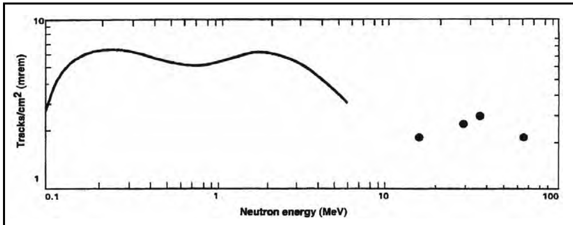
Figure A-5. Neutron energy response of NTS TED (Allen and Schoengold 1995).
