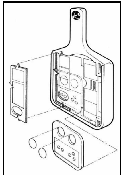
Figure 6-2. Security badge for NRDS TLD.
