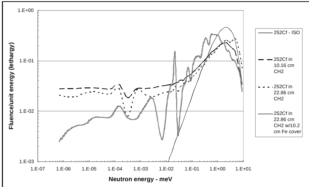
Figure A-8. Lethargy neutron spectra for ^{252}\text{Cf} with various thickness moderators (IAEA 2001).
