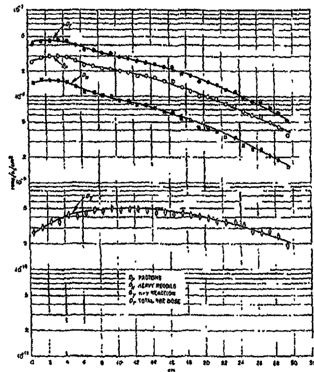
FIGURE 3B. RBE dose (rems) from 7.5-Mev neutron beam.
