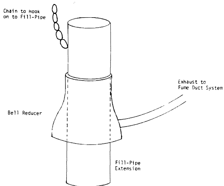
Figure 4. Fill-Pipe Extension
