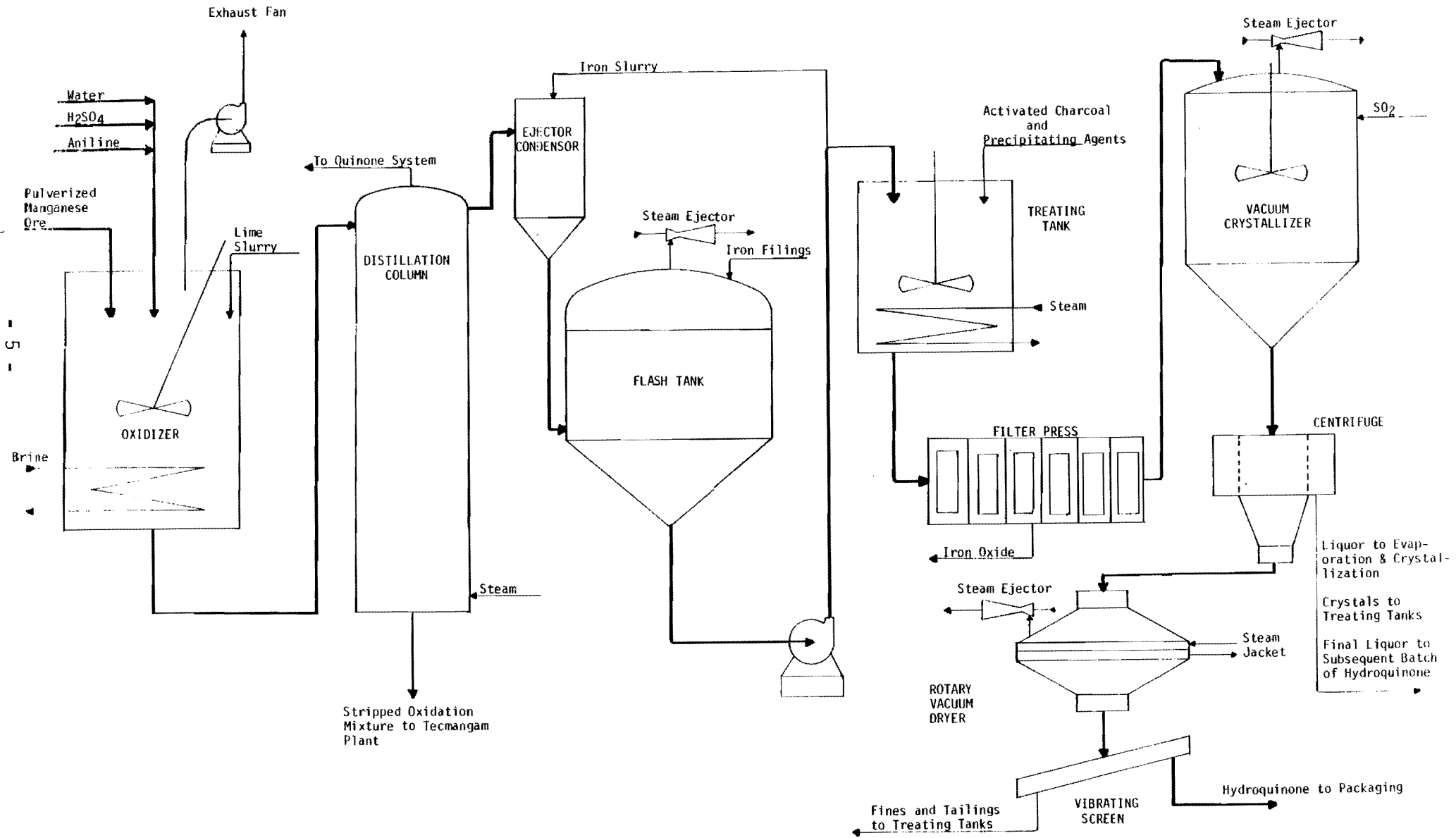
Figure 2. Hydroquinone Manufacture
