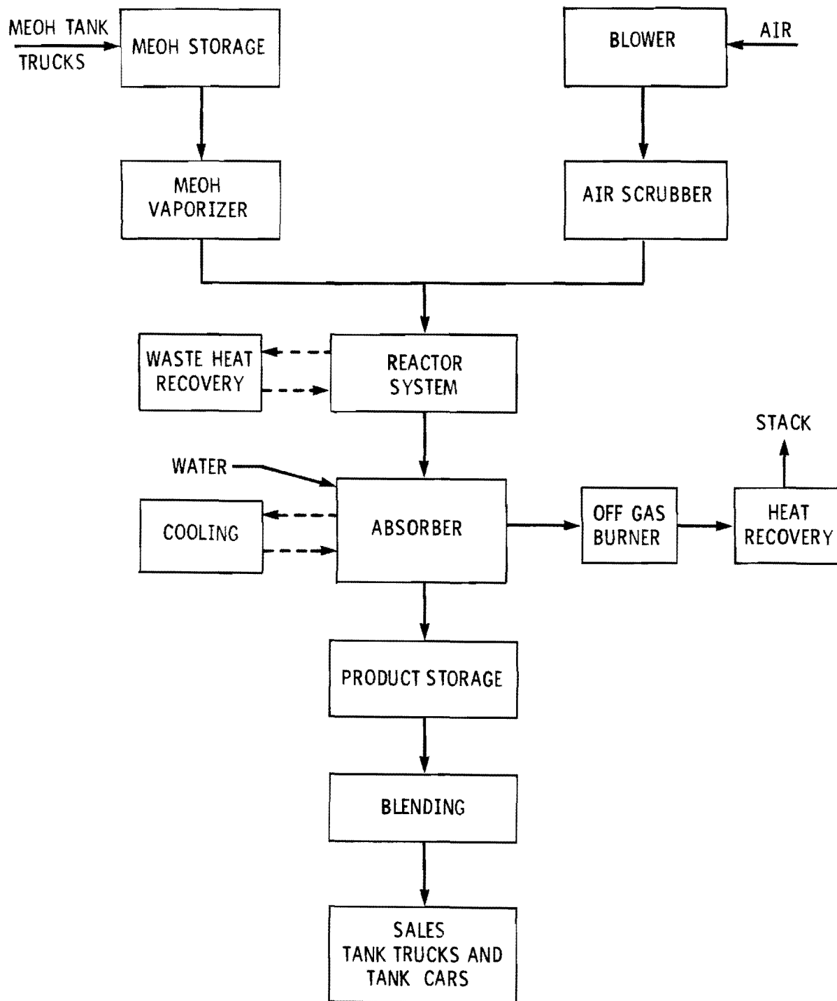
Figure 2. Formaldehyde process - block flow diagram.
