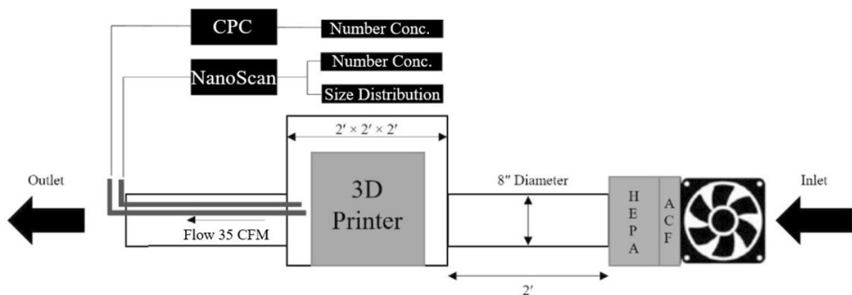
Figure 6: 3D printer emission test chamber schematic showing dimensions and sampling equipment. Schematic by NIOSH.
