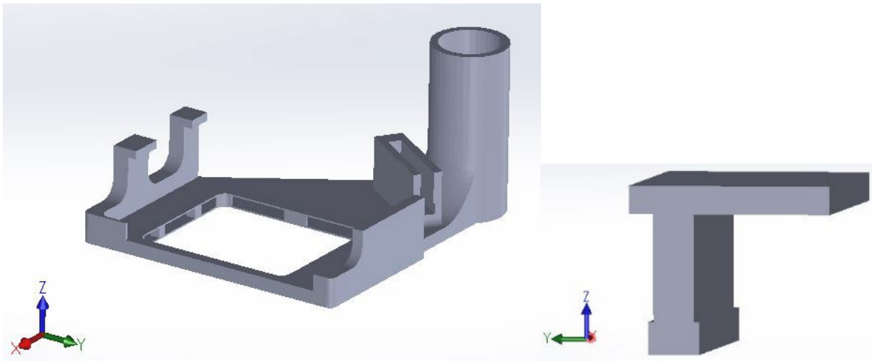
Figure 4: LEV control designed to remove emissions from the point of origin for 3D Printer B. Left is the main body of the control, right is the tab to secure the part to the extruder head. Design by NIOSH.
