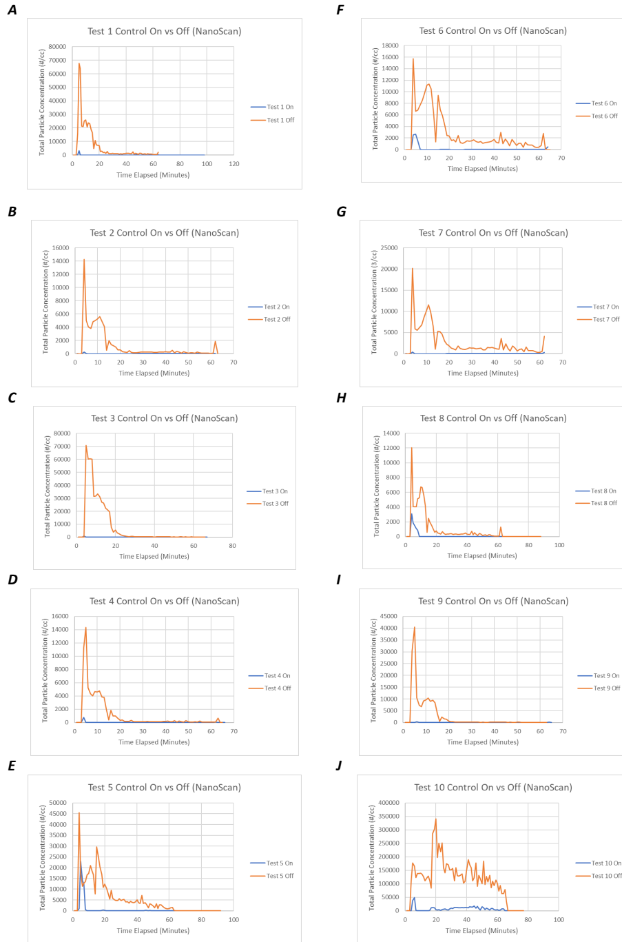
Figure 10: 3D Printer B – total particle concentration vs time with and without the custom retrofitted engineering control.
