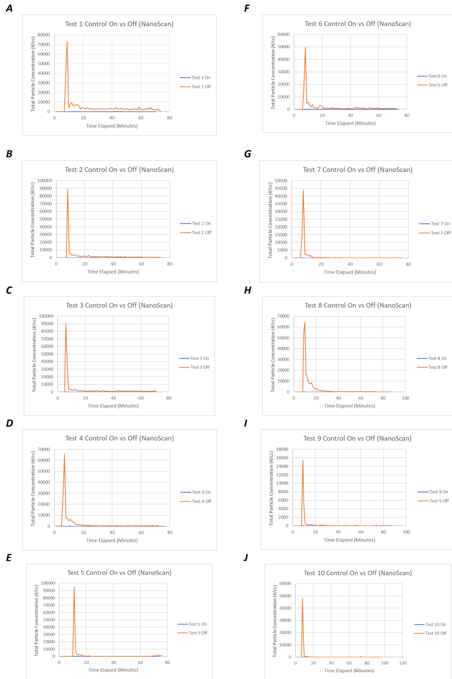
Figure 9: 3D Printer A - total particle concentration vs time with and without the custom retrofitted engineering control.
