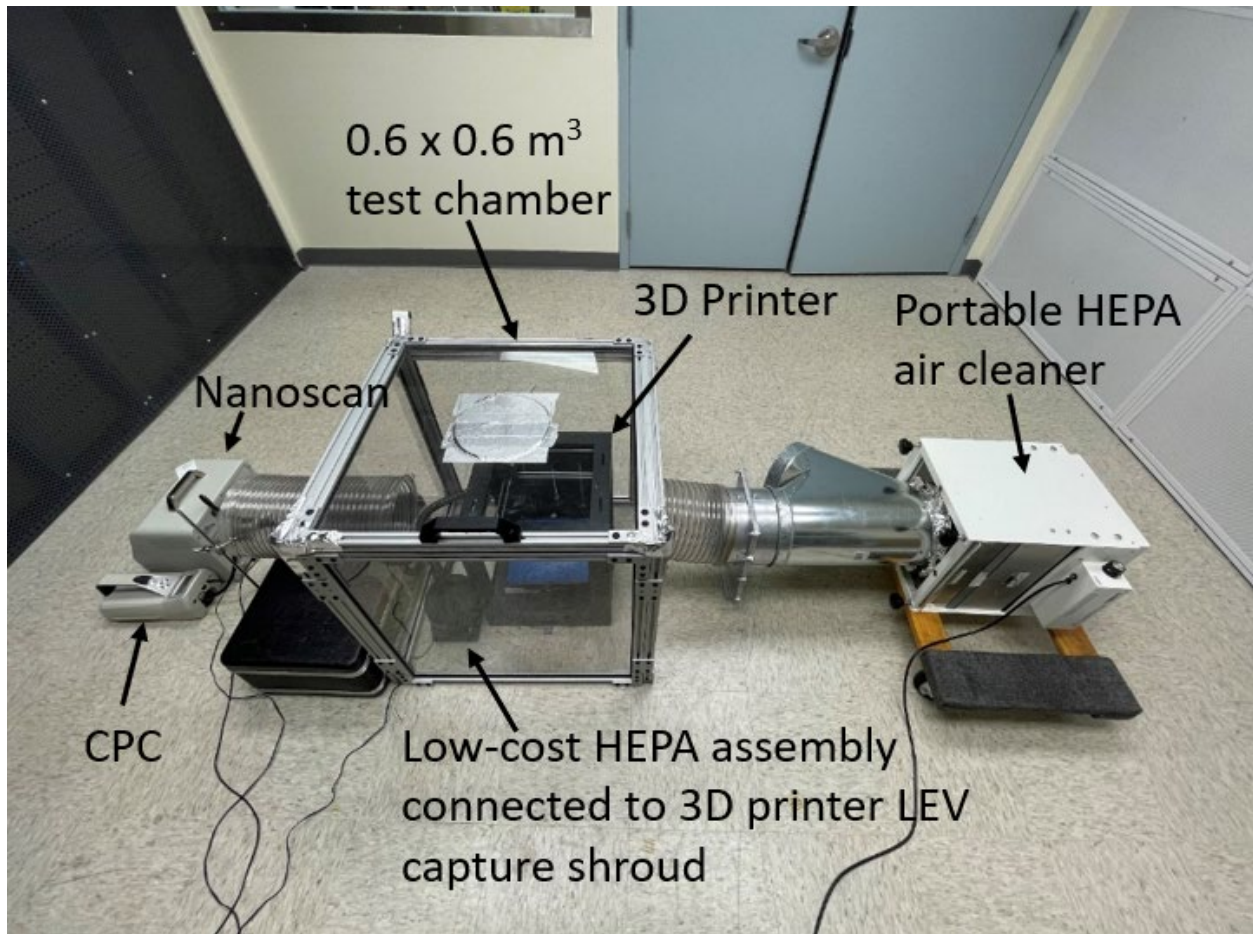
Figure 7: Actual 3D printer emission test chamber with 3D Printer A and sampling equipment. Photo by NIOSH.
