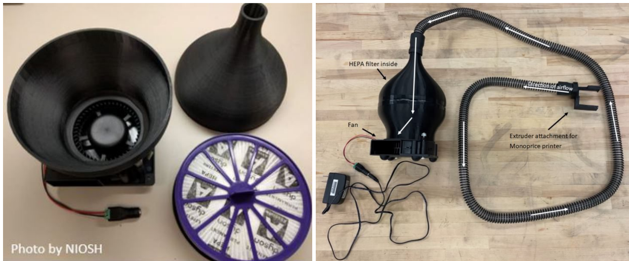
Figure 3: Low-cost HEPA air cleaner assembly (left). Right picture shows the HEPA assembly connected to a 3D printed LEV capture shroud. The HEPA filter is 14 cm (5.5 in) in diameter and 2.5 cm (1 in) in thickness. Photos by NIOSH.
