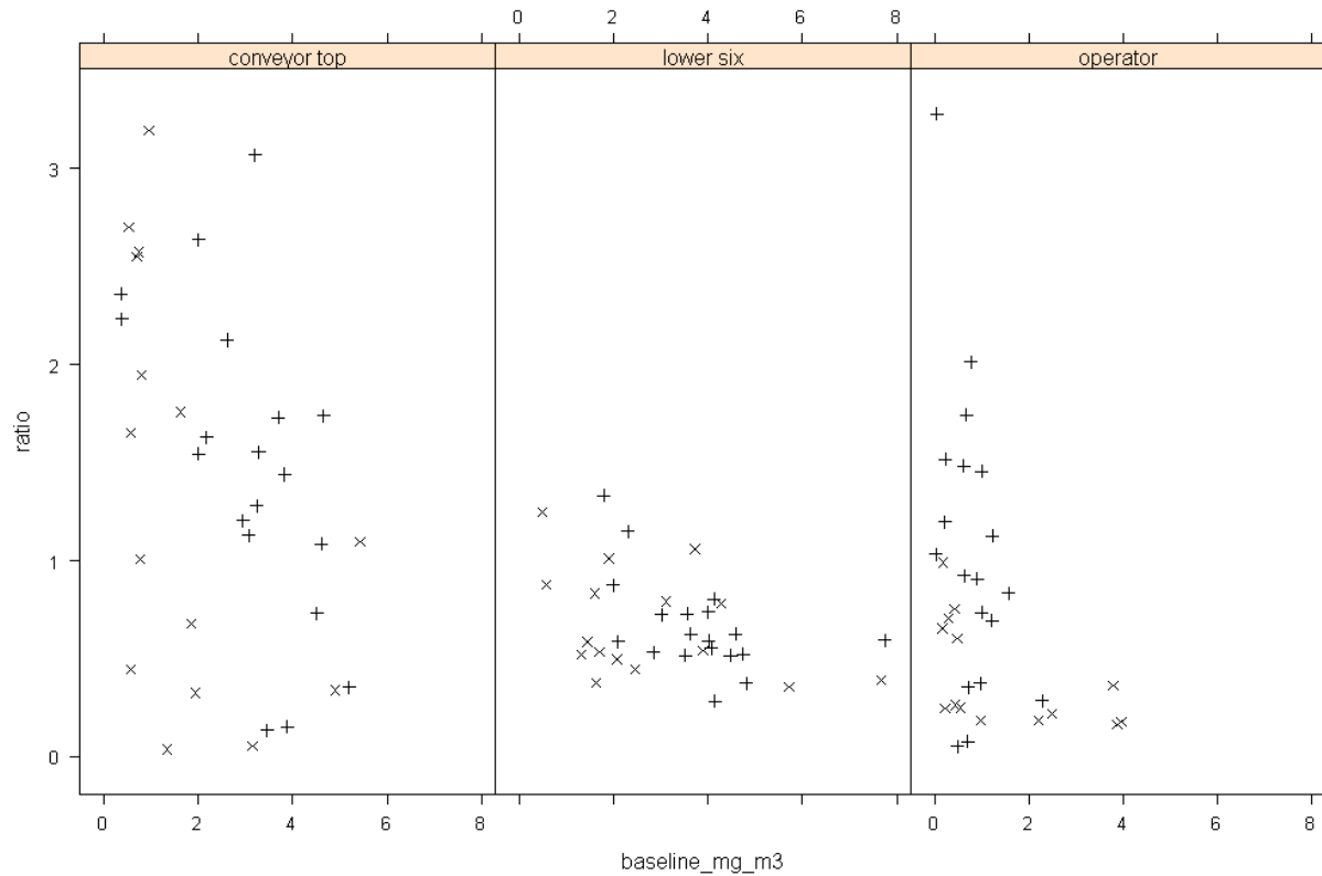
Figure 2: 2010 ("x") and 2012("+") wet drum to baseline ratios at the three locations, plotted versus baseline concentrations in \text{mg}/\text{m}^3 . (One large baseline conveyor top value is not shown.)
