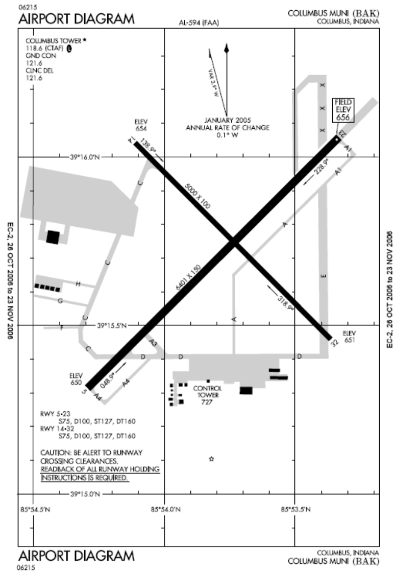
Figure A1 - Airport Diagram. Runway Construction Took Place on Runway 5-23, Below the Intersection with Runway 14-32 [FAA 2010].
