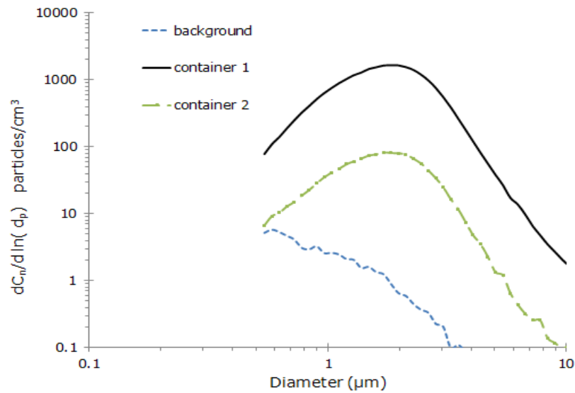
Figure 10. The graphene platelets recovered from the process had aerodynamic diameters larger than 0.5 μm. During disconnection of Containers 1 and 2, the mass concentrations estimated from the APS number concentrations were 9 and 0.4 mg/m 3 on 9/26.
