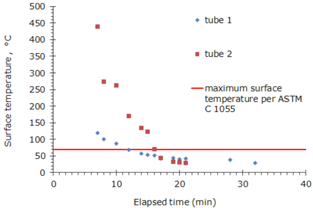
Figure 19. Surface temperature change over time on the glass tubes for the post-treatment process. Cooling time can be used to mitigate the risk of a contact burn. This suggests that about 20 minutes is needed to minimize the risk of a burn.
