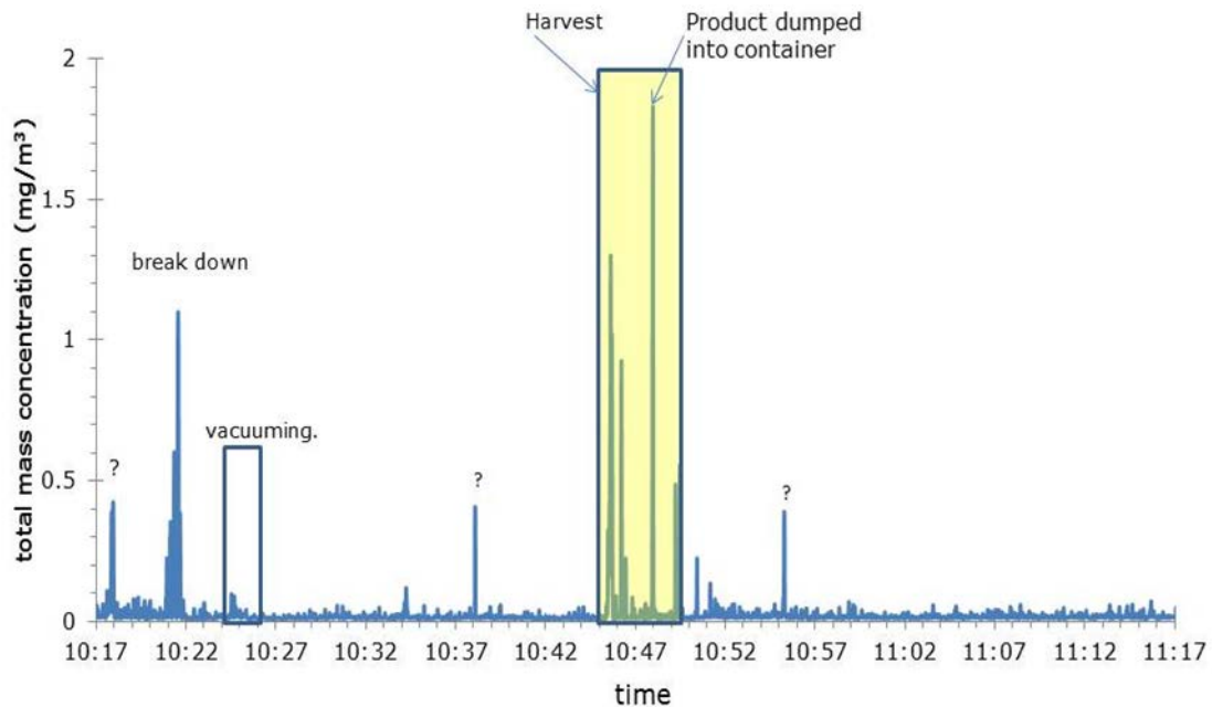
Figure 21. Monitoring data for the post-treatment process (annotations were based upon notes).
