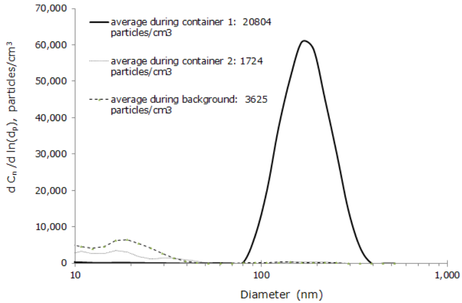
Figure 9. Size-dependent concentrations measured with the FMPS during container removal on 9/26.
