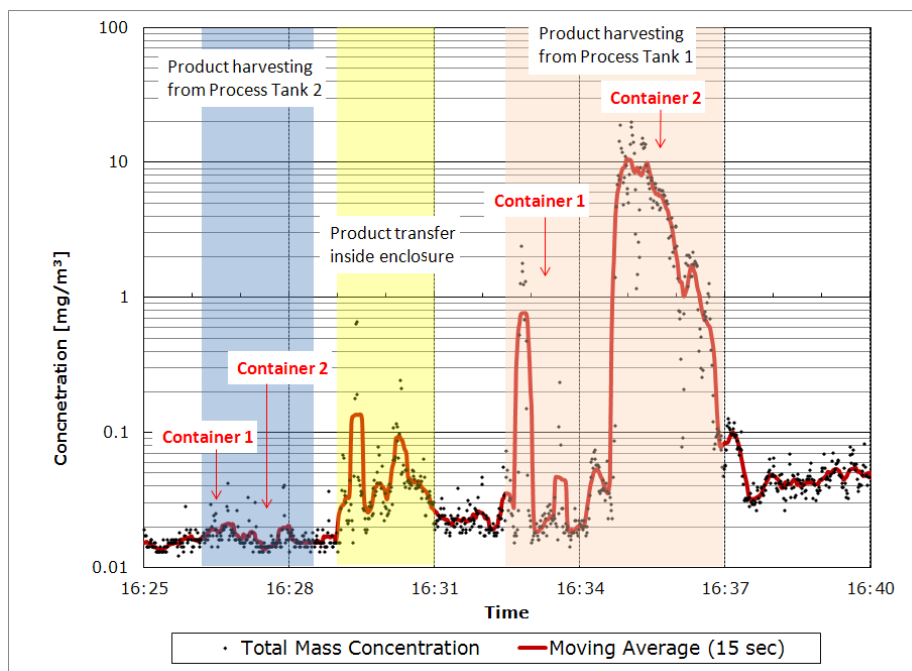
Figure 5. Previous monitoring data of product harvesting from two refining process tanks, as measured by the DustTrak aerosol monitor on September 29, 2010.
