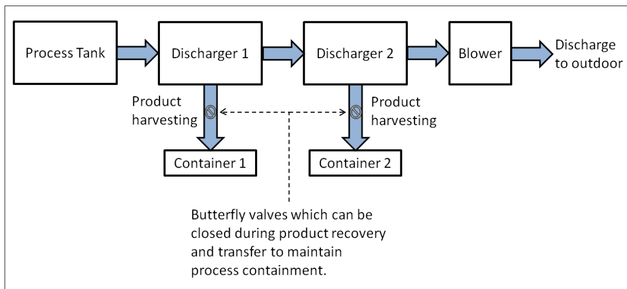
Figure 4. Process Tank 2 used for the refining process. This equipment is smaller than Process Tank 1. It has design features that should minimize dust emissions.
