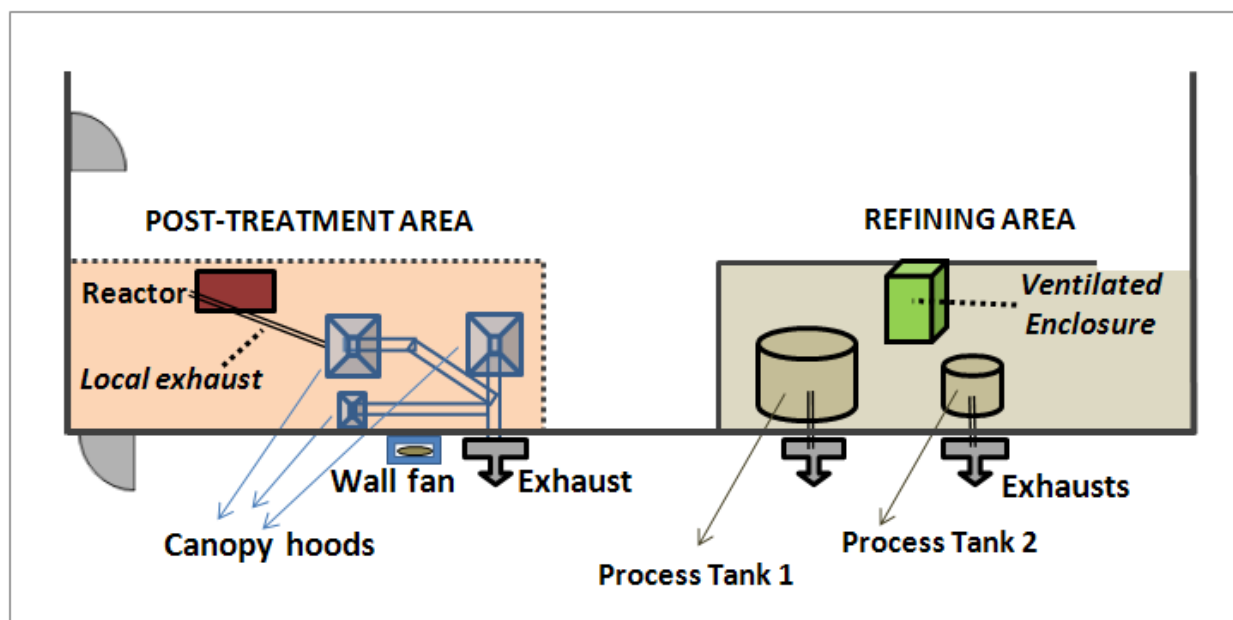
Figure 2. Layout of the production areas at the study site.
