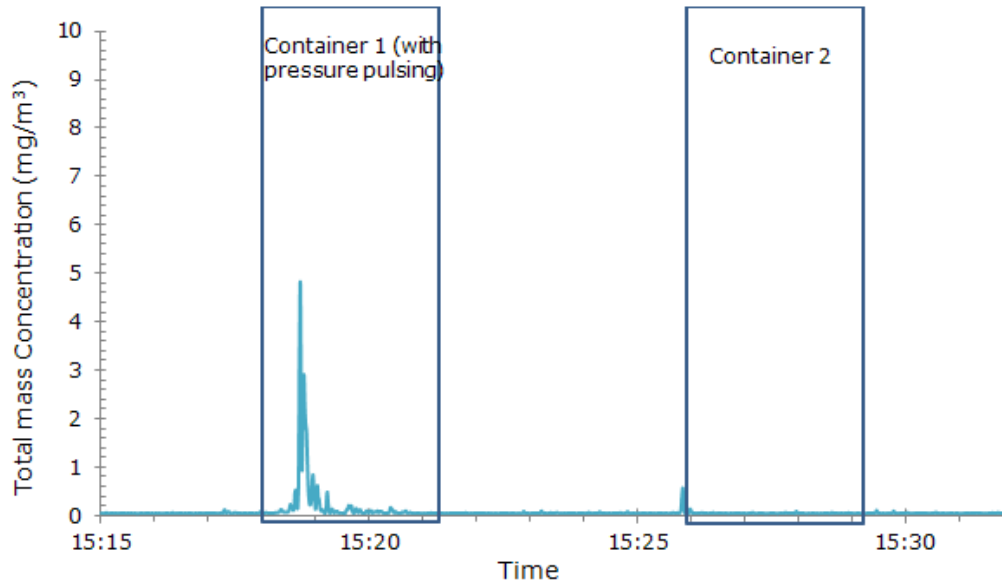
Figure 11. Results from DustTrak with a 30-minute delay in product harvesting. Pressure pulsing was on until Container 1 was removed.
