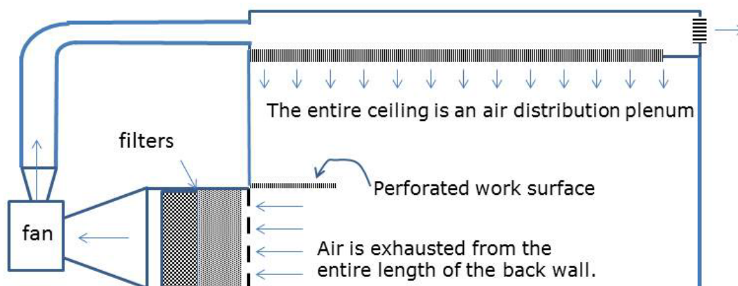
Figure 22. Conceptual sketch of downflow-ventilated booth or room. The airflow from the ceiling should be 35–100 fpm [Heinonen et al. 1996; Floura and Kremer 2008].
