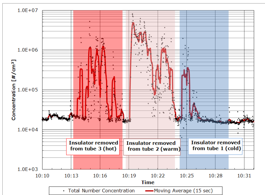
Figure 6. Previous sampling results from the tubes with different cooling times during the post-treatment process, as monitored by the FMPS on September 30, 2010.
