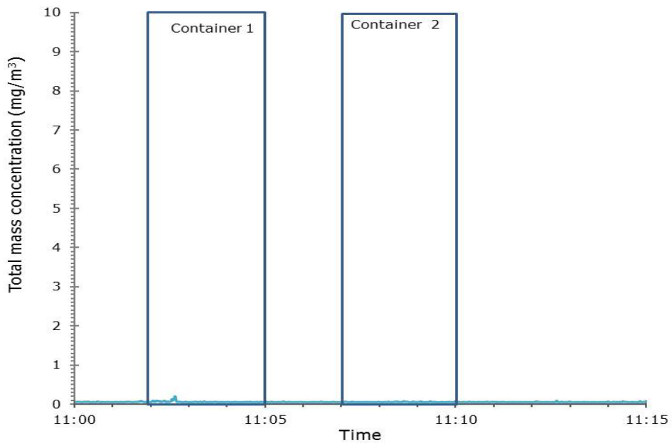
Figure 12. Results from DustTrak with repetition of a 30-minute delay in product harvesting. The process, including pressure pulsing, was completely shut down before removal of Container 1.
