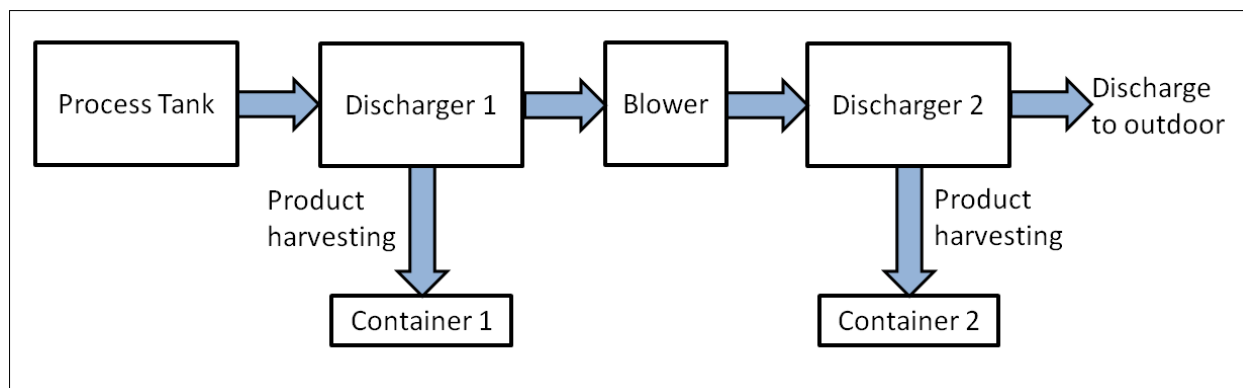
Figure 3. Process Tank 1 used for the refining process. Products are harvested by manually unlocking containers.
