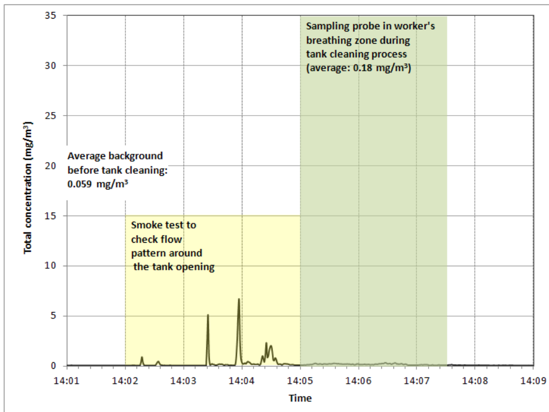
Figure 14. Real-time monitoring of nanomaterials released during the maintenance task for Process Tank 1 on 09/28. The task was performed with the fan on to exhaust fugitive nanomaterials.
