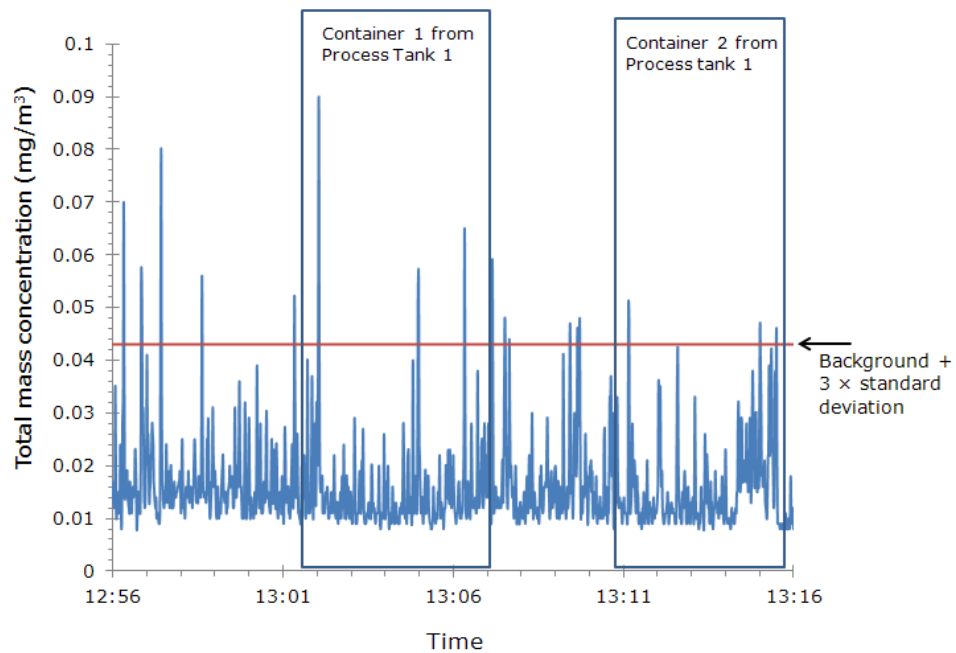
Figure 15. Dust exposures during the first weigh-out session.
