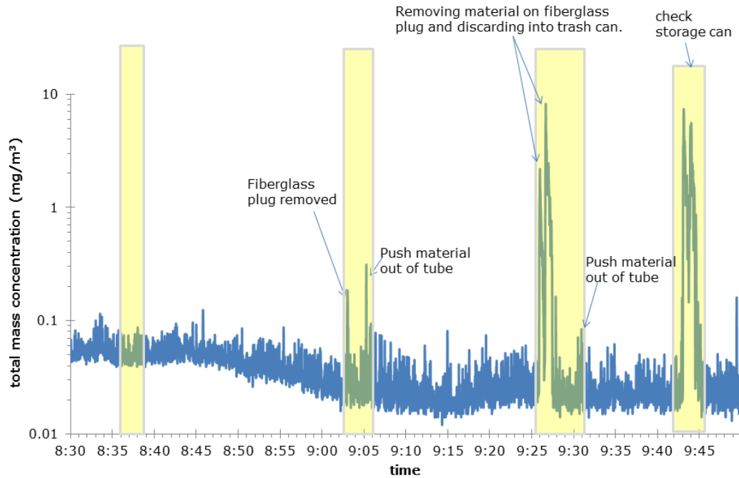
Figure 20. Monitoring data for the post-treatment process (annotations were based upon videotape).
