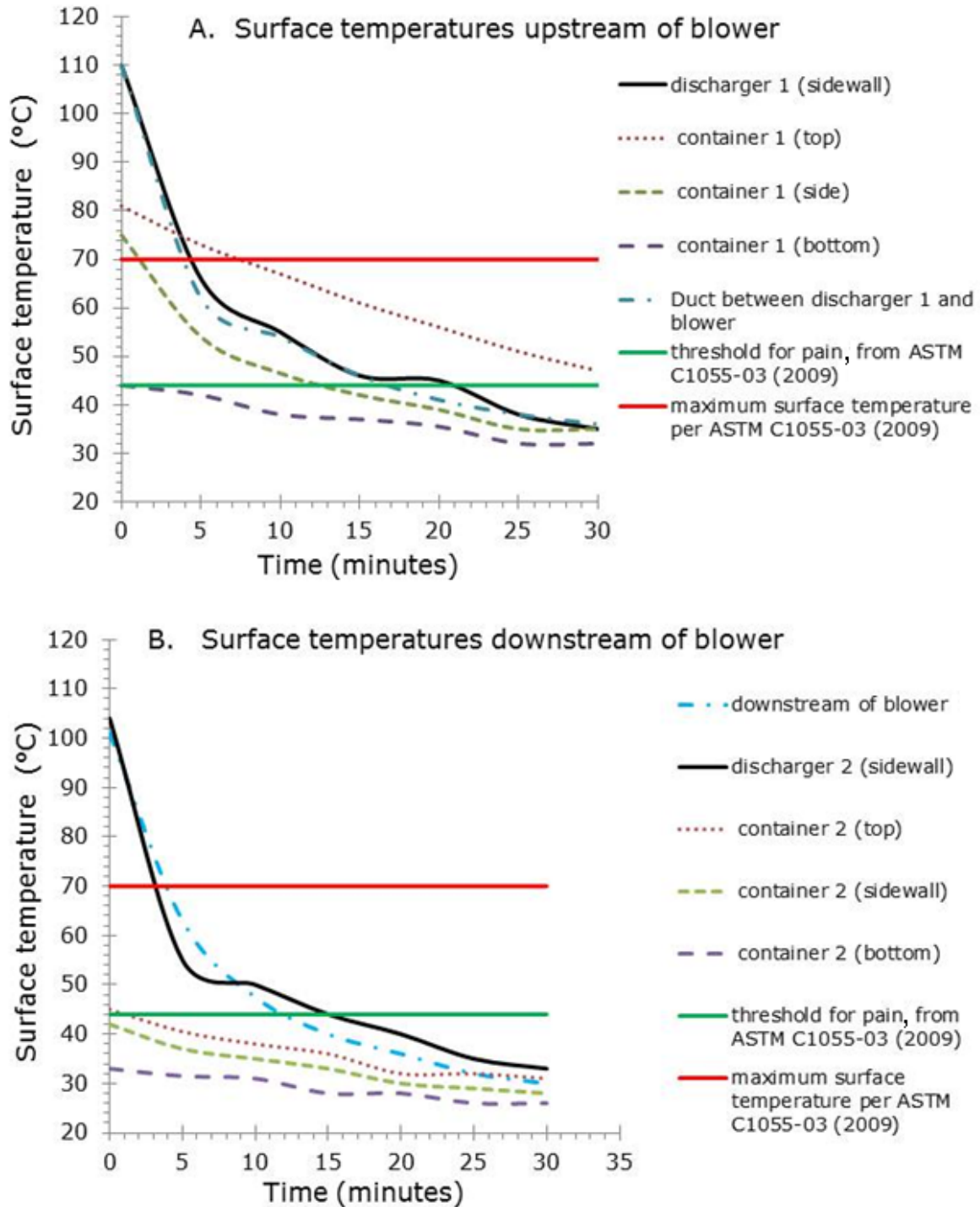
Figure 18. Surface temperature changes on the refining equipment. The temperatures at time = 0 minutes are steady temperatures at the end of the process.
