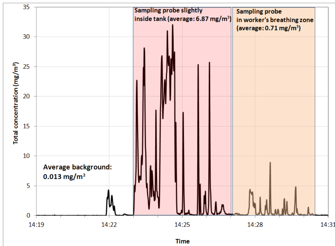
Figure 13. Real-time monitoring of nanomaterials released during maintenance cleaning of Process Tank 1 on 09/15. The regular task procedures were followed, with no engineering controls.
